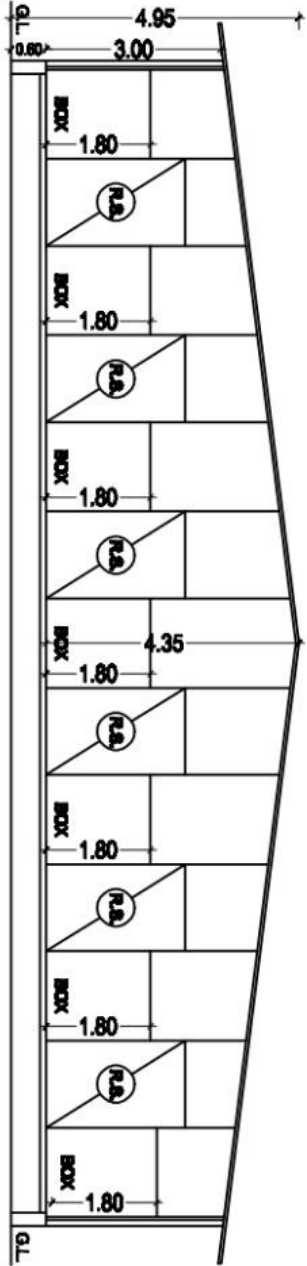
ONION STORAGE SHED - 02 SECTION AT - AA SCALE - 1:200
